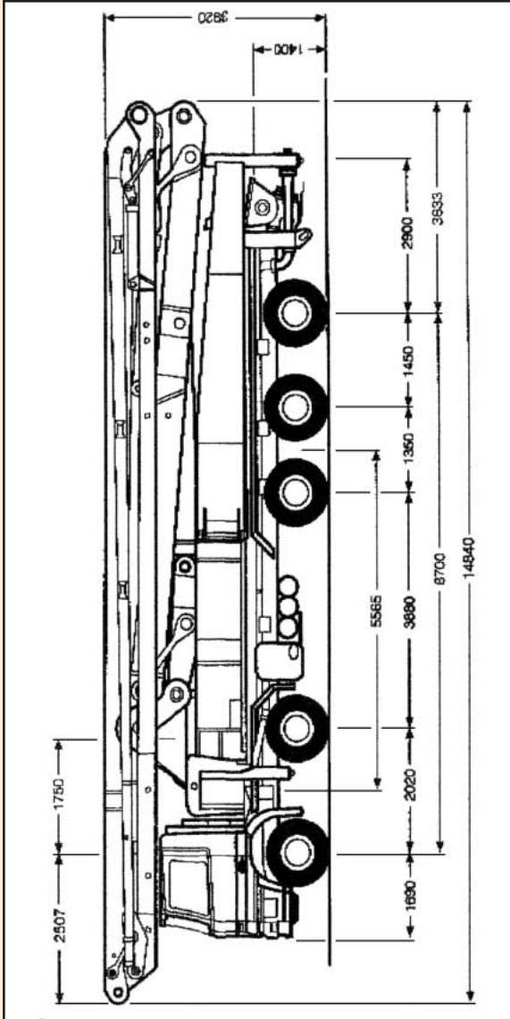
58 Metre Concrete Pump.
