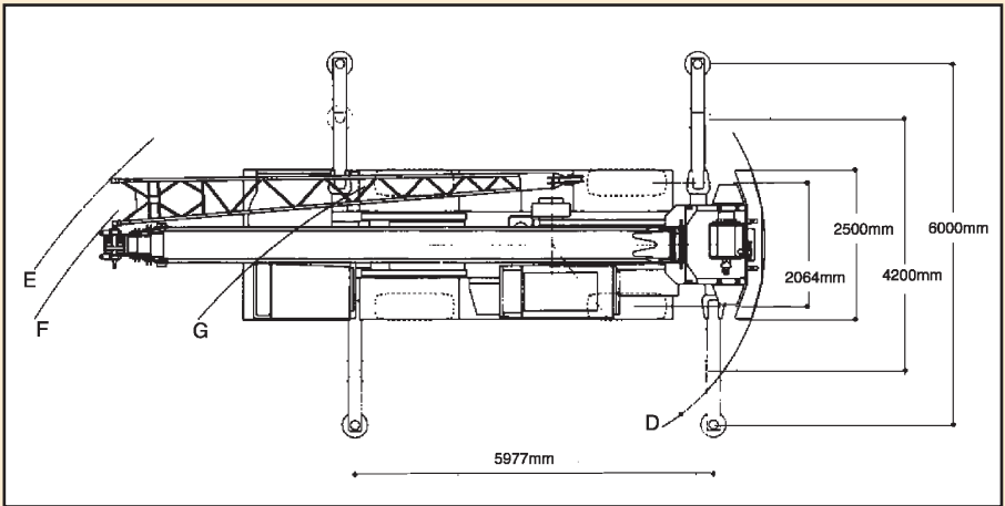
CRANE PLAN
