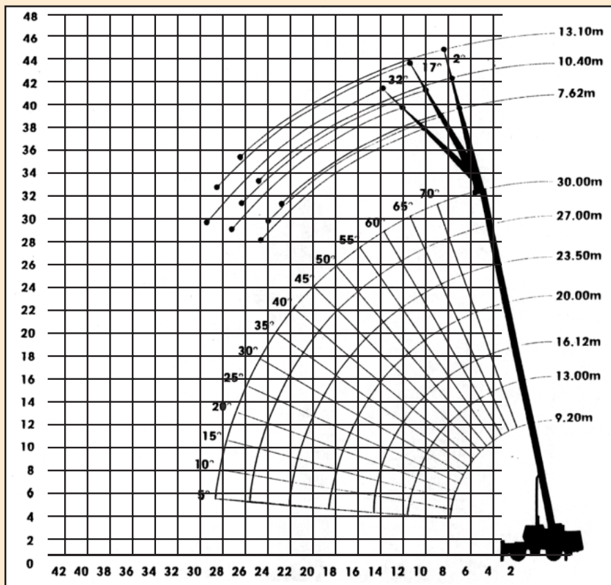
WORKING RANGE
